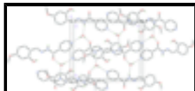
Fig. 2. The crystal packing diagram of compound (I), viewed along the a axis. Hydrogen bonds are shown as dashed lines.
