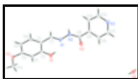
Fig. 1. The molecular structure of compound (I), with 30% probability displacement ellipsoids for non-H atoms.
